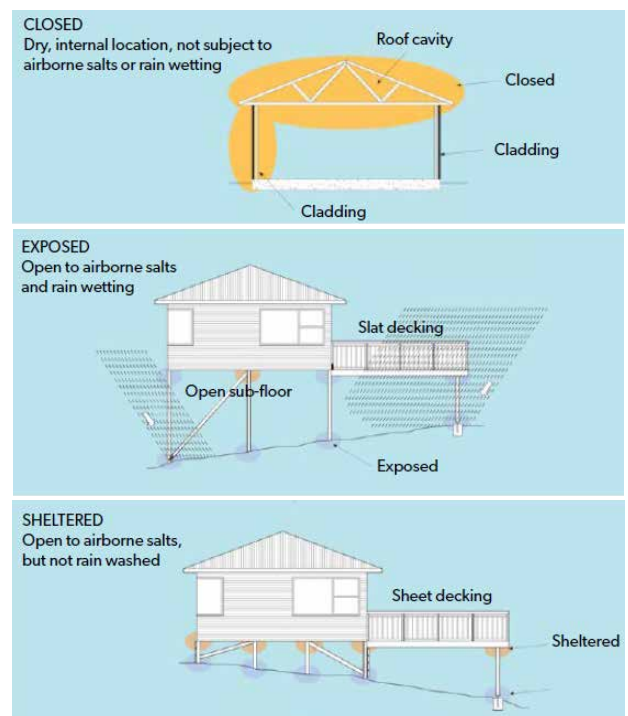
Fig 4.3(a & b) NZS 3604:2011
