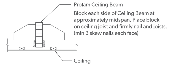
SECTION THROUGH CEILING BEAM
