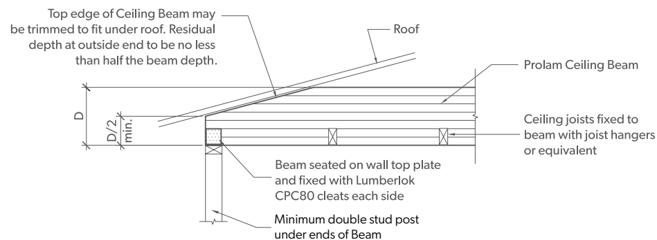
ELEVATION AT END OF CEILING BEAM
