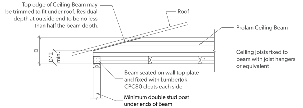
ELEVATION AT END OF CEILING BEAM
