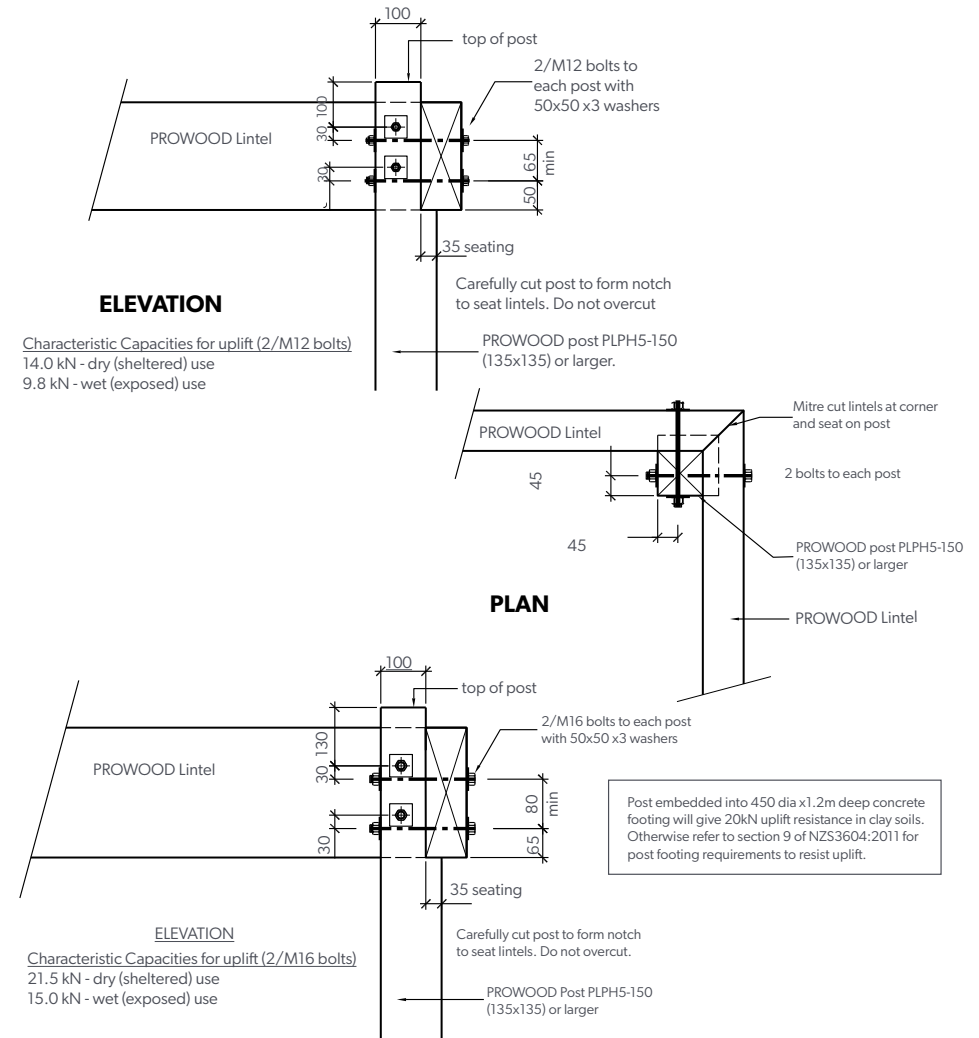
CORNER POST - LINTEL CONNECTION DETAIL
