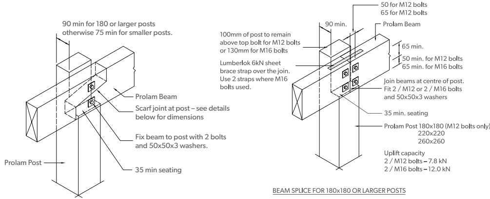
SCARF JOINT AT POSTS
