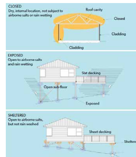
Fig 4.3(a & b) NZS 3604:2011
