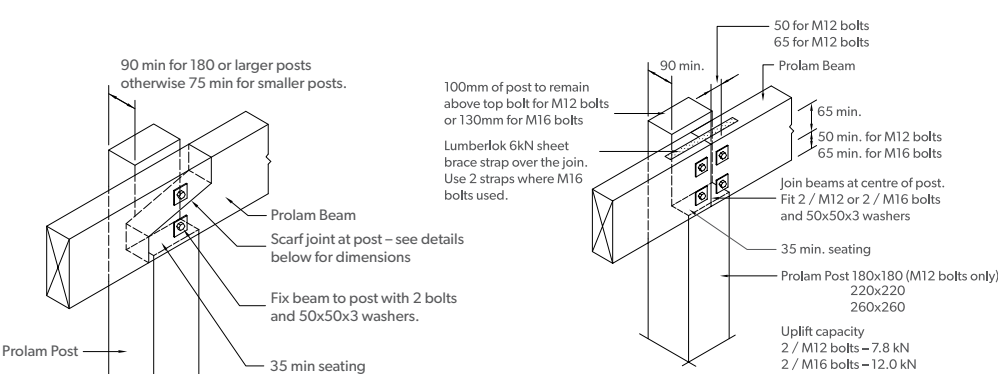
SCARF JOINT AT POSTS
