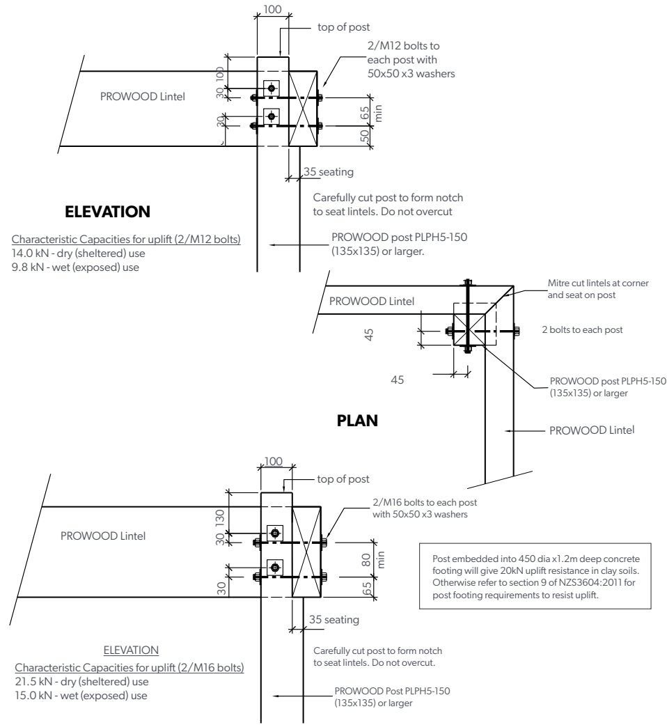
CORNER POST - LINTEL CONNECTION DETAIL
