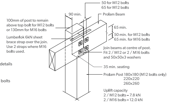
BEAM SPLICE FOR 180x180 OR LARGER POSTS
