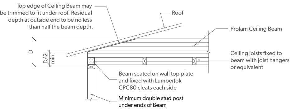
ELEVATION AT END OF CEILING BEAM
