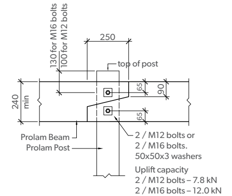
SCARF JOINT FOR 240 OR LARGER BEAMS
