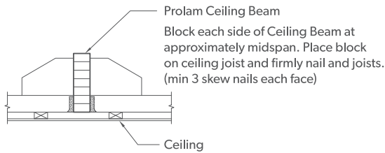
SECTION THROUGH CEILING BEAM
